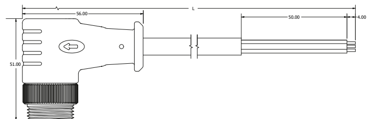
MALE ANGLED
