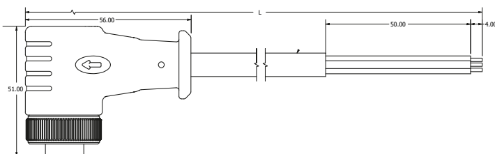
FEMALE ANGLED
