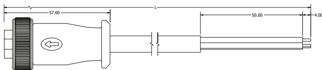
FEMALE STRAIGHT
