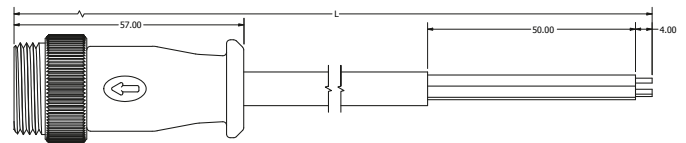
MALE STRAIGHT
