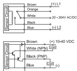
AC Receiver, Diffuse & Retro
